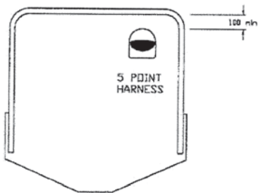
HELMET CLEARANCE
