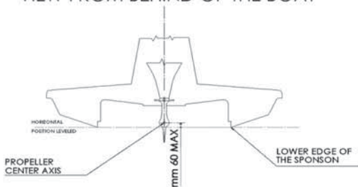
VIEW FROM BEHIND OF THE BOAT
