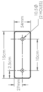
ANTI-SUBMARINE BELT ALTERNATE MOUNTING PLATE
